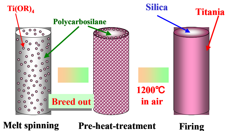
Fig. 3. Fundamental concept of our photocatalytic fiber
