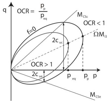
Figure 18: The Niemunis and Grandas-Tavera model [40]. M_{CS_e} and M_{CS_e} are the slopes of the CSL for triaxial compression and extension, respectively. M_\Omega denotes the slope of the CSL by the current \Omega .
