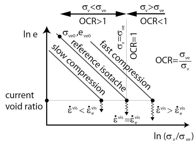
Figure 10: Isotaches concept.
