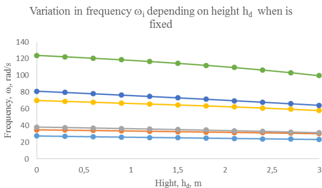
Fig. 2. Variation in frequency \omega_i depending on height h_d when w_w is fixed
