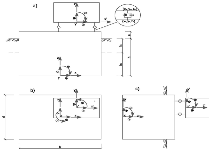
Fig. 1. Model of block-type foundation sunk in ground and machine resting on foundation: a) front view, b) top view, c) side view
