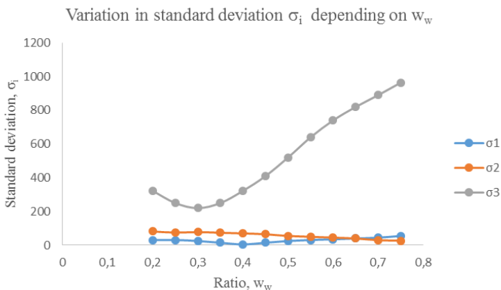
Fig. 4. Variation in standard deviation \sigma_i depending on w_w
