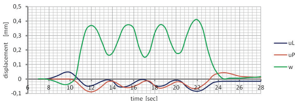
Fig. 10. Deflections of the shell crown during the passage of two locomotives
