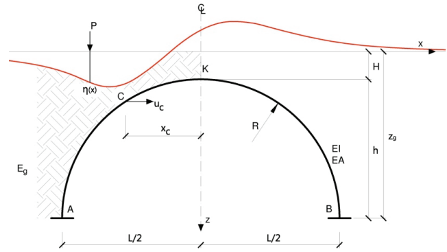
Fig. 2. Geometrical characteristics of a circumferential segment of a soil-steel structure and the influence function of shell horizontal displacement
