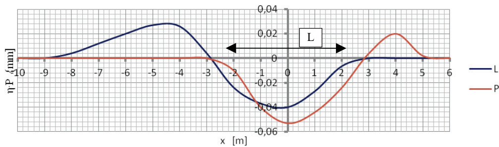
Fig. 13. Influence lines of the horizontal displacement of the “L” and “P” side of the shell determined on the basis of measurements
