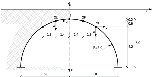
Fig. 4. Scheme of the circumferential segment of the soil-steel structure and the location of the point analysed
