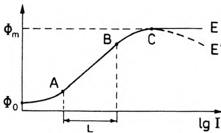
Fig. 5. Exposure curve for the photographic materials (AB – linear range, CE' – solarization range).
