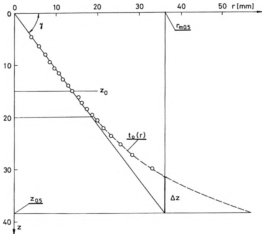
Fig. 10. Transform t_p(r) of the diffraction image created by the pulverisation cone of the main injector of K 108-767 type at the fuel forcing pressure p_t = 10 MPA.
