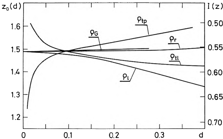
Fig. 12. Dependence of the zero order place z_0 of the function R_\rho(z) on the relative standard deviation d for five statistical distributions ( \rho_l(D) – logarithmic normal distribution, \rho_{tl}(D) – triangular distribution ( \gamma > 0 ), \rho_G(D) – Gaussian distribution, \rho_r(D) – uniform distribution, \rho_{tp} – triangular distribution ( \gamma < 0 )).
