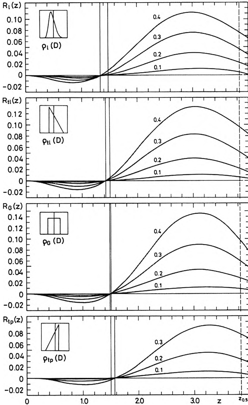
Fig. 11. Functions R_\rho(z) = I_\rho(z) - I_\rho(z) for statistical distributions \rho(D) ; \rho_l(D) – logarithmic normal distribution, \rho_{tl}(D) – triangular distribution ( \gamma > 0 ), \rho_G(D) – uniform distribution, \rho_{tp}(D) – triangular distribution ( \gamma < 0 ).
