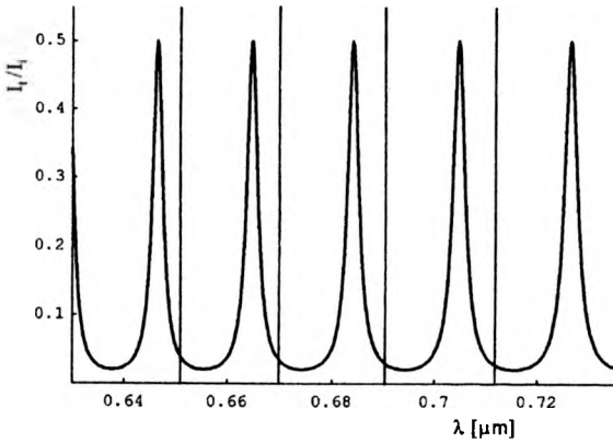
Fig. 5. Shift in ordinary spectrum of FPF with W602 for the case when chromatic dispersion is fitted to sodium yellow line ( T = 294 K).
