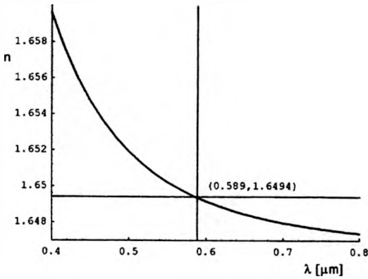
Fig. 2. Chromatic dispersion in W602 mixture fixed for sodium yellow line (extraordinary refractive index in W602 mixture, T = 294 K).
