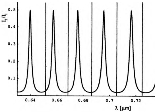
Fig. 3. Shift in FPF spectrum for chromatic dispersion fitted to yellow line of sodium. Ticks are placed at positions of measured peaks (extraordinary spectrum in W602 mixture, T = 294 K).
