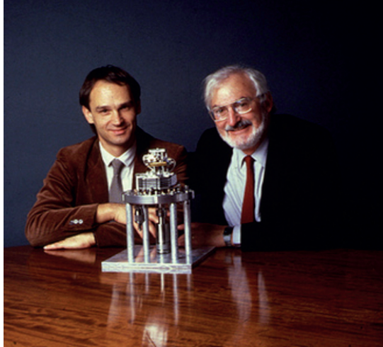
Rysunek 2. G. Binnig i H. Rohrer wraz z STM [8] Figure 2. G. Binnig and Rohrer with STM [8]
